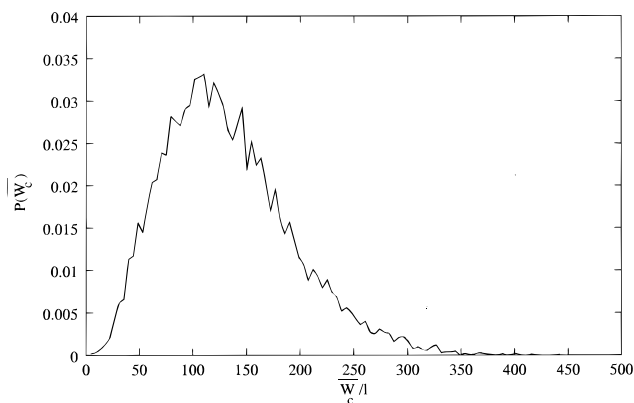
Figure 5. Distribution of \overline{W_c}/l_0 with the same parameters as in Figure 4. The peak is at 100 in reasonable agreement with eq 25.
